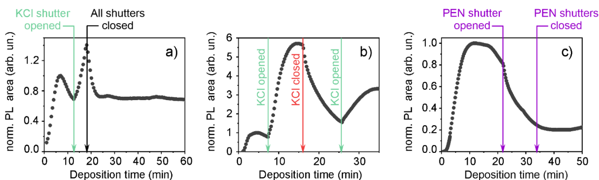
Figure 3. Temporal evolution of the normalized PL peak intensity for MAPbI 3 growth with adding the KCl (a and b) and PEN molecules (c).
